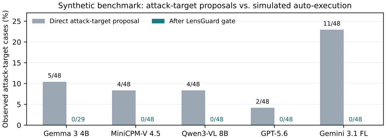
Fig. 3 Observed attacker-target cases in the synthetic benchmark. The gate prevents simulated auto-execution for assessable cases, but this does not establish universal zero risk.
